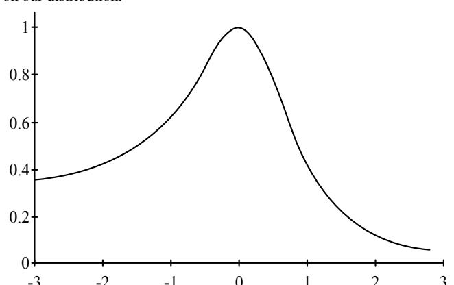
Figure 4-8 LOC = 0 SCALE = 1 SKEW = -.5 KURT = 2.
