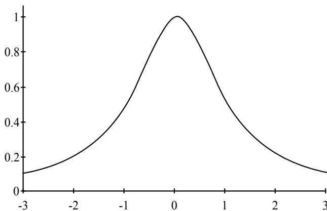
Figure 4-2 LOC = 0 SCALE = 1 SKEW = 0 KURT = 2.
