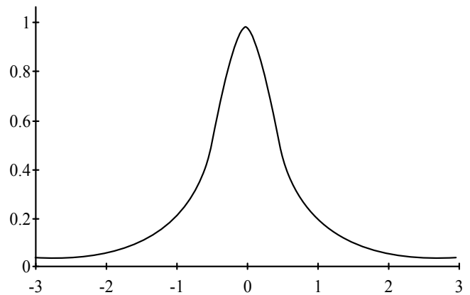
Figure 4-7 LOC = 0 SCALE = 2 SKEW = 0 KURT = 2.
