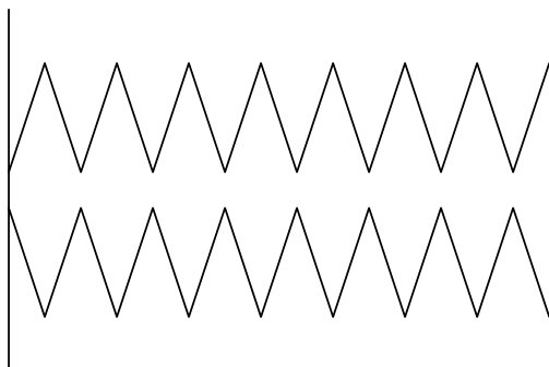
Figure 1-3 Negative correlation ( r = -1.00 ).
