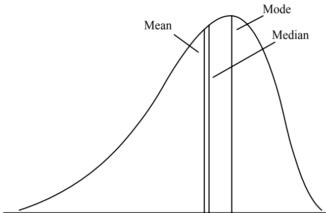
Figure 3-3 Skewness alters location.
