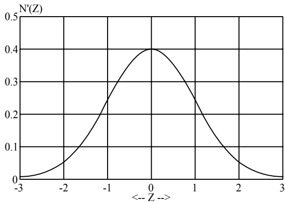
Figure 3-7 The Normal Probability density function.
