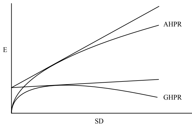
Figure 7-5 AHPR, GHPR, and their CML lines.
