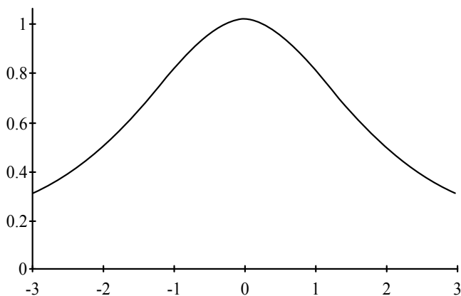
Figure 4-6 LOC = 0 SCALE = .5 SKEW = 0 KURT = 2.
