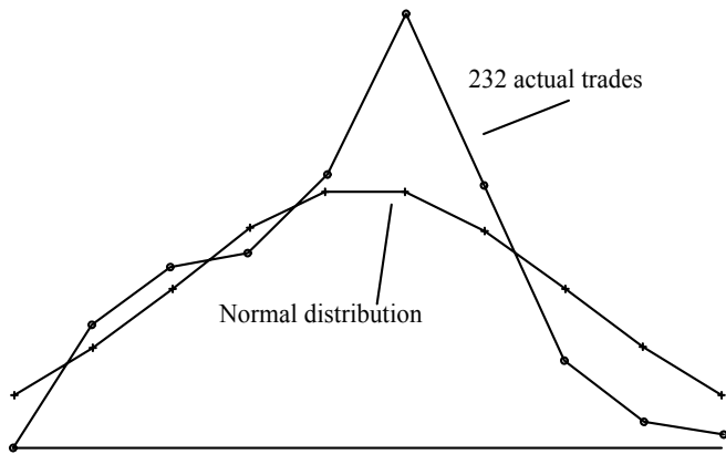
Figure 3-16 232 individual trades in 10 bins from -2 to +2 sigma versus the Normal Distribution.
