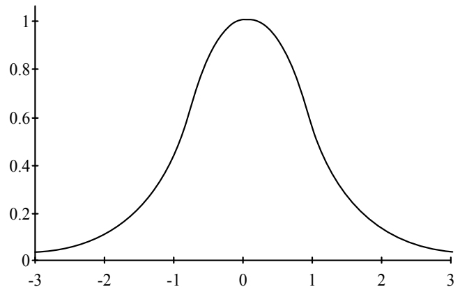
Figure 4-4 LOC = 0 SCALE = 1 SKEW = 0 KURT = 3.
