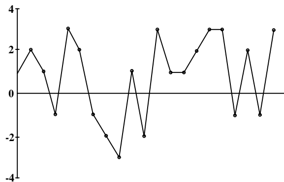
Figure 1-4 Individual outcomes of 21 trades.
