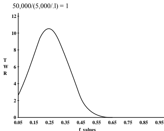
Figure 1-1 20 sequences of +2, -1.
