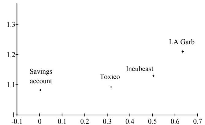
Figure 6-1 The upper-right quadrant of the Cartesian plane.
