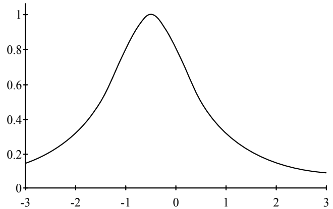
Figure 4-3 LOC = -.5 SCALE = 1 SKEW = 0 KURT = 2
