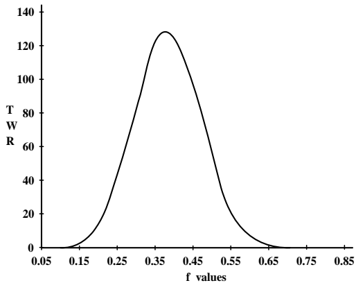
Figure 1-6 20 sequences of +5, -1.
