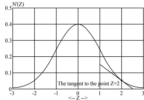
Figure 3-13 N''(Z) giving the slope of the line tangent tangent to N'(Z) at Z = +2 .
