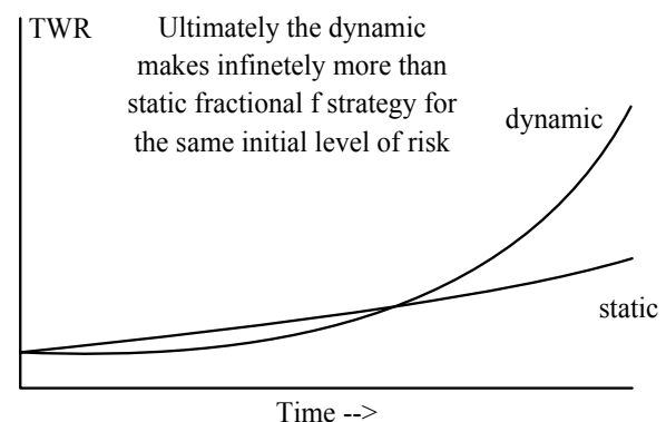
Figure 8-1 Static versus dynamic fractional f.
