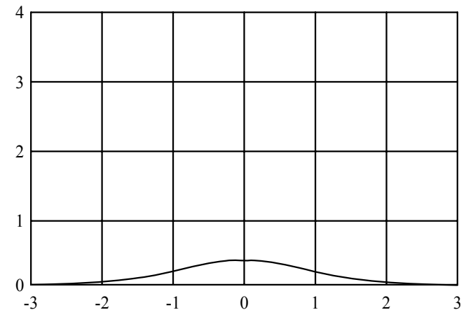
Figure 3-14 The real shape of the Normal Distribution.
