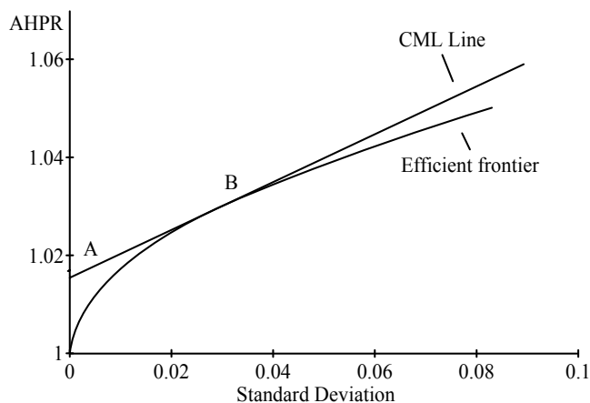
Figure 7-1 Enhancing returns with the risk-free asset.
