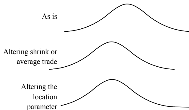
Figure 4-12 Altering location parameters.
