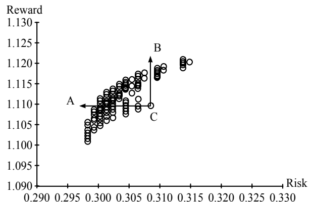
Figure 1-7 Modern portfolio theory.
