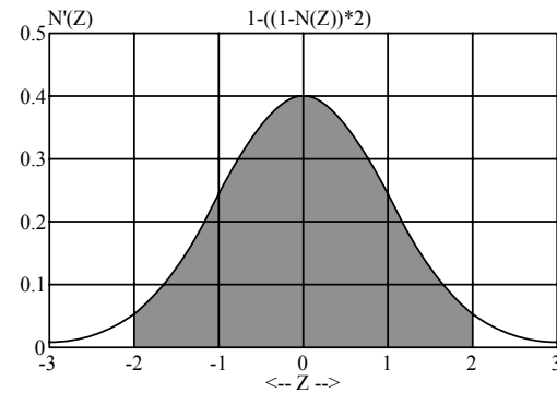
Figure 3-10 A two-tailed probability of an event being +or-2 sigma.
