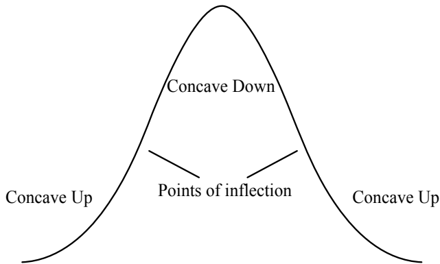
Figure 4-11 Points of inflection on a bell-shaped distribution.
