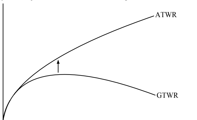
Figure 7-3 The efficient frontier with/without reinvestment
