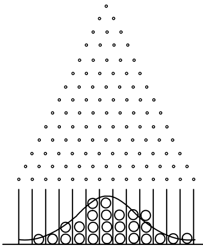
Figure 3-5 Galton's board.
