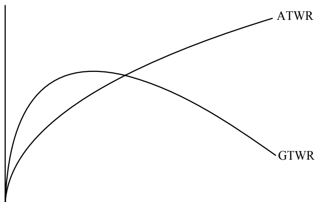
Figure 7-4 The efficient frontier with/without reinvestment.
