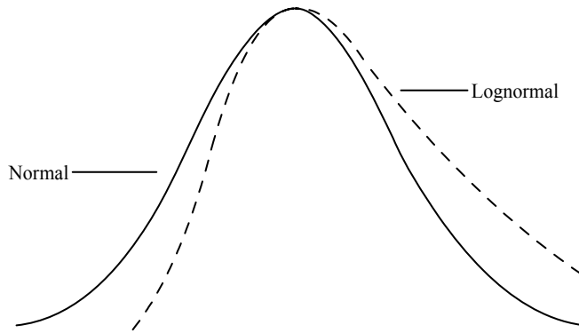
Figure 3-15 The Normal and Lognormal distributions.
