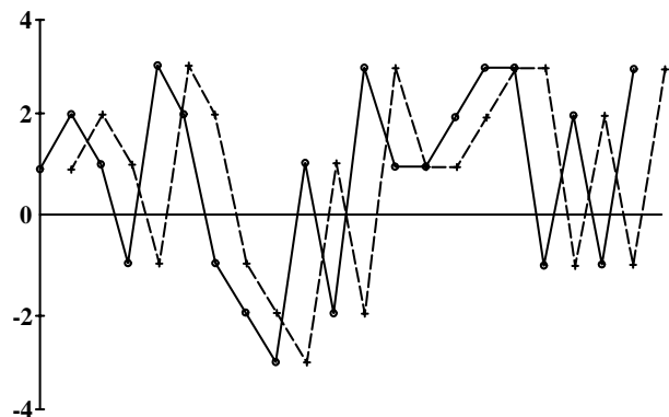
Figure 1-5 Individual outcomes of 21 trades skewed by 1 trade.
