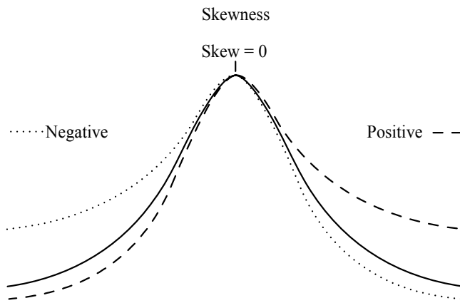
Figure 3-2 Skewness
