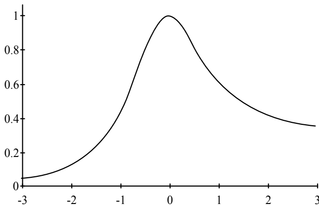
Figure 4-9 LOC = 0 SCALE = 1 SKEW = +.5 KURT = 2.
