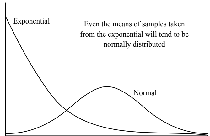
Figure 3-6 The Exponential Distribution and the Normal.
