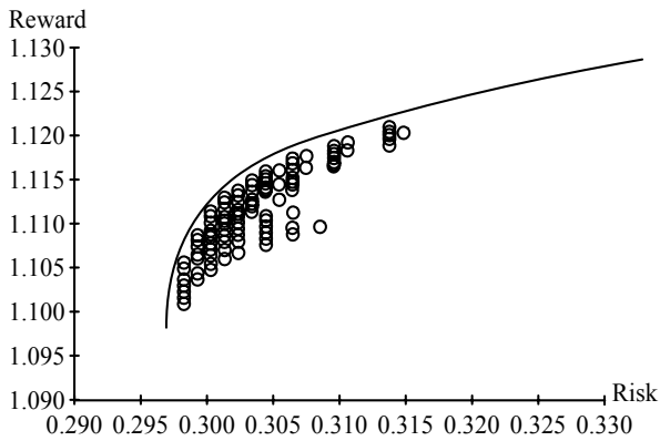
Figure 1-8 The efficient frontier
