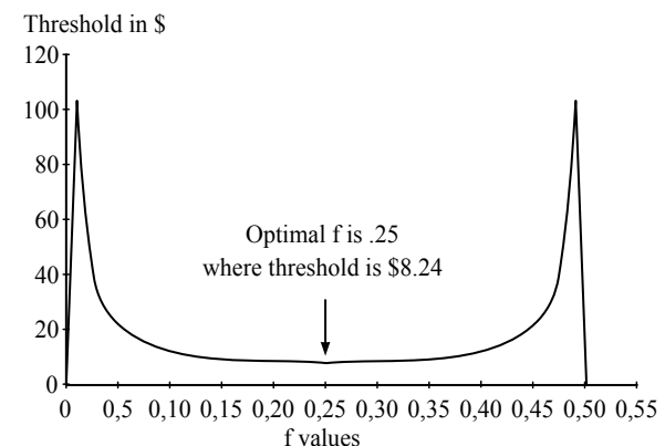
Figure 2-1 Threshold to the geometric for 2:1 coin toss.
