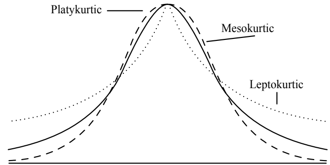
Figure 3-4 Kurtosis.
