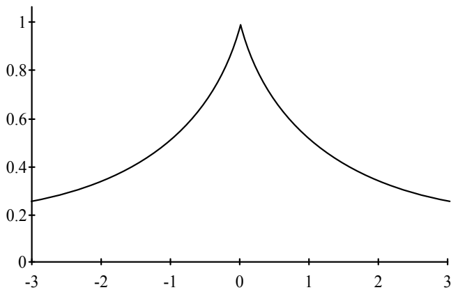
Figure 4-5 LOC = 0 SCALE = 1 SKEW = 0 KURT = 1
