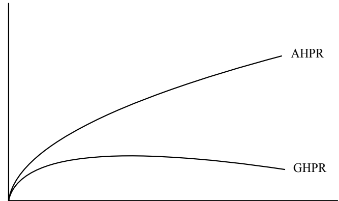
Figure 7-2 The efficient frontier with/without reinvestment
