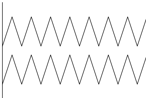
Figure 1-2 Positive correlation ( r = +1.00 ).
