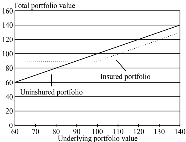
Figure 8-2 Portfolio insurance.
