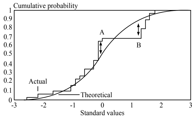
Figure 4-1 The K-S test.
