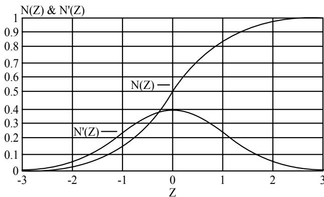
Figure 3-8 Equation (3.21) showing probability with Z = +2.
